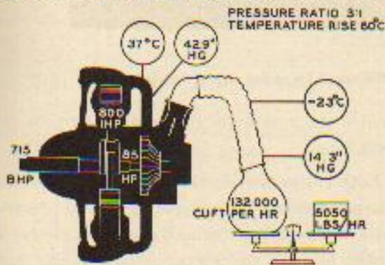
FULL THROTTLE CHARACTERISTICS AT 19000 FT.
