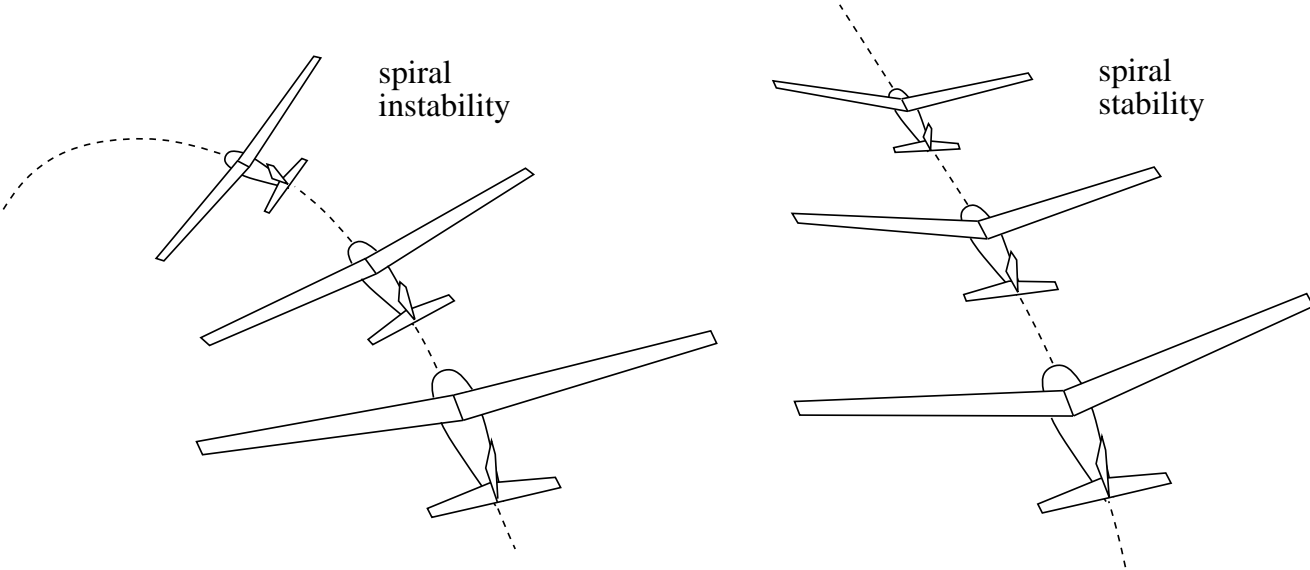
Figure 6: Spiral instability and spiral stability, depending on amount of dihedral.
