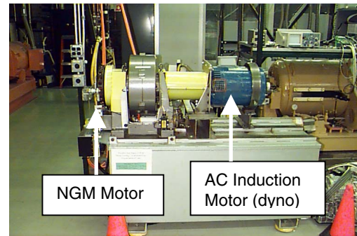
Figure 2: Portable Motor Test Stand
