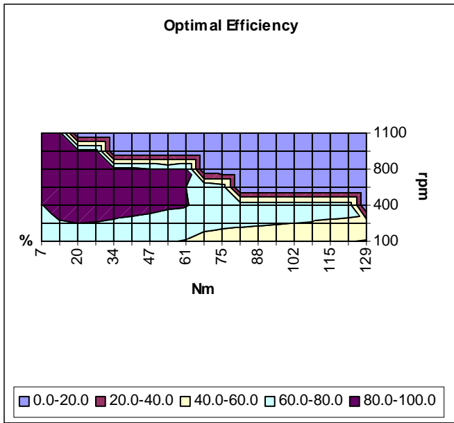
Figure 10: Optimal efficiency
