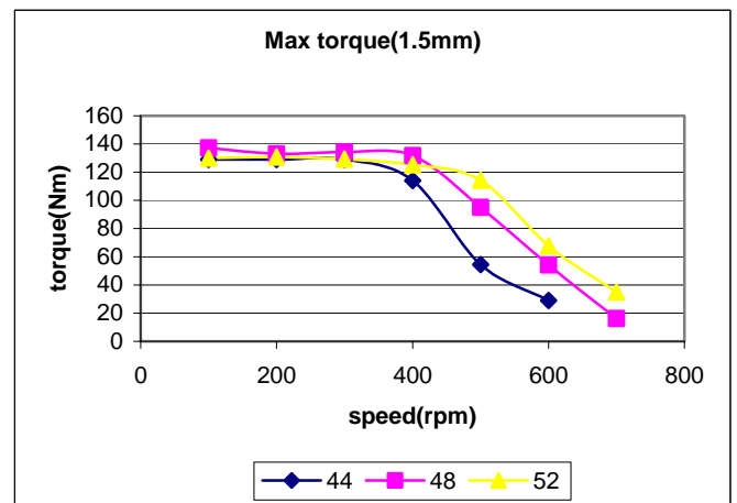
Figure 27: Maximum Torque at Different Input Voltages (1.5-mm gap)
