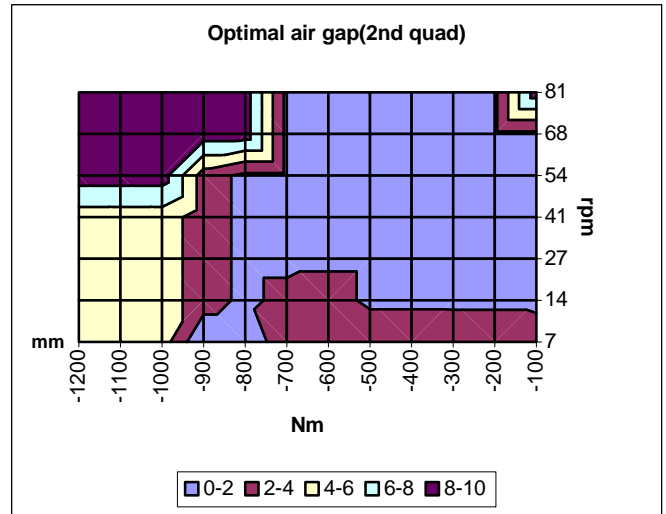
Figure 22: Optimal Efficiency
