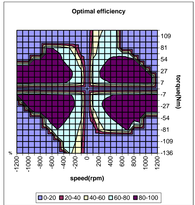
Figure 26: Optimal Efficiency (fourth quadrant)
