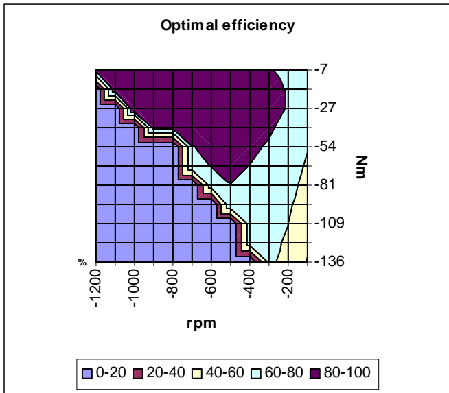
Figure 19: Optimal efficiency
