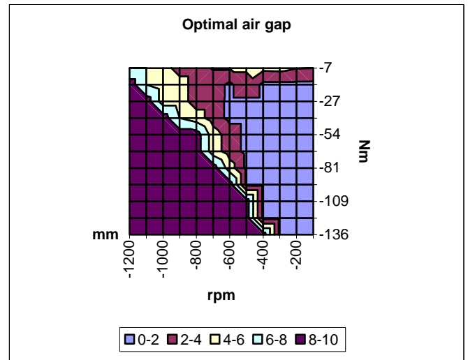
Figure 18: Optimal Air Gap
