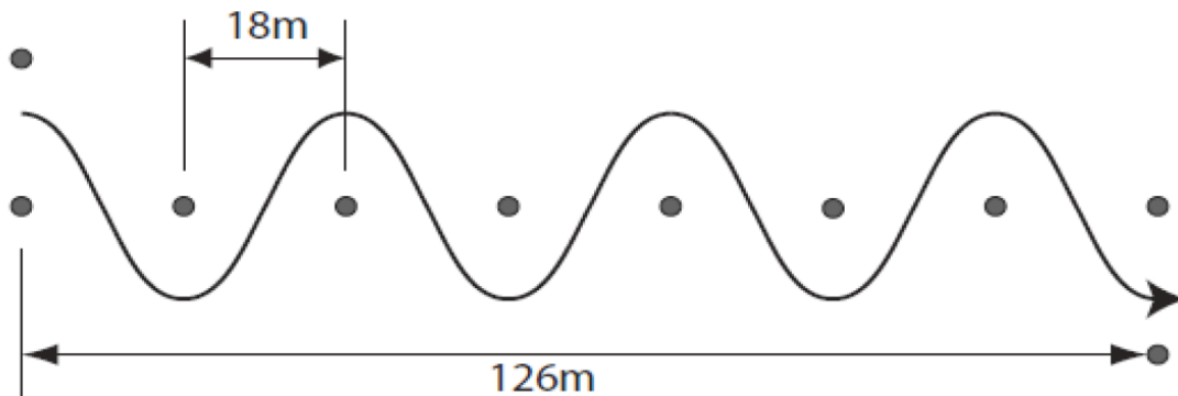
Figure 6-2 Slalom Course Layout
