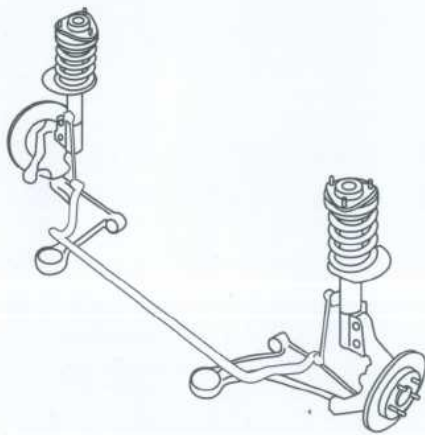
McPHERSON STRUT
